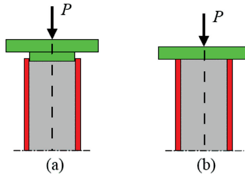
Figure 4. A schematic view of the application of the axial load for (a) tubed RC column and (b) typical CFT column
