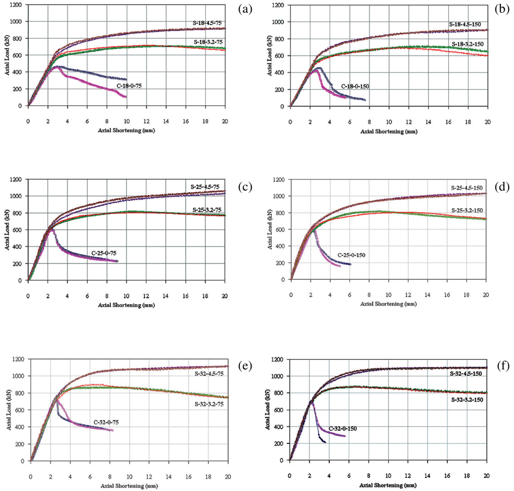
Figure 6. Axial load versus axial shortening of the RC and tubed RC columns
