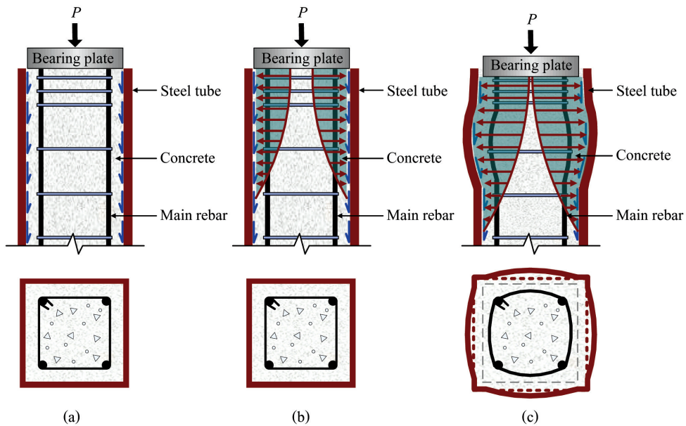
Figure 7. A schematic view of transferring mechanism of the applied load near the top end of the tubed RC column (a) at the early stage, (b) during linear elastic behavior and c.) during nonlinear behavior
