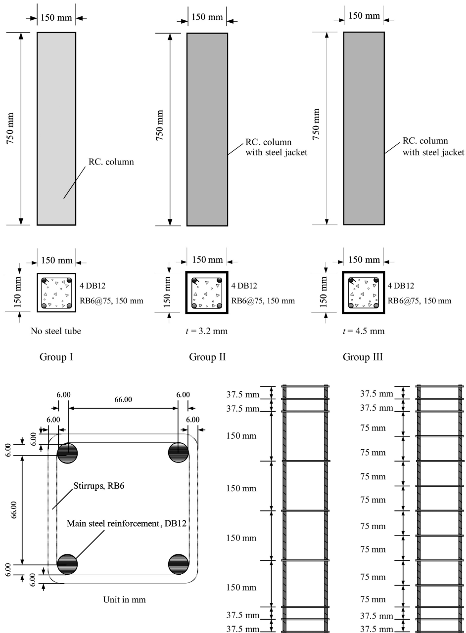
Figure 2. A schematic view of the details of the test specimens
