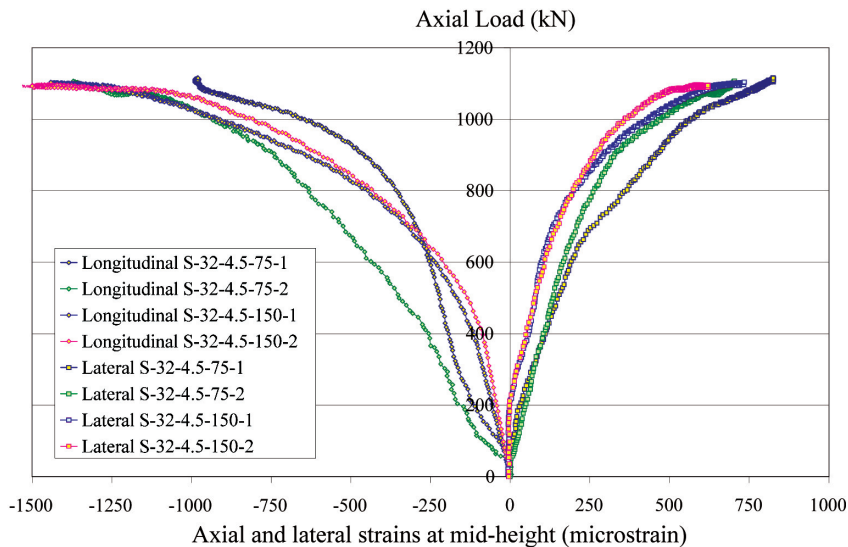
Figure 8. Axial load versus axial and lateral strains at the mid-height of the tubed RC column specimen S-32-4.5
