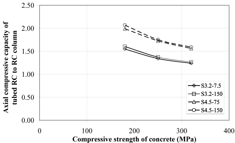
Figure 11. N_{c,exp} / N_{c,RC} ratio versus compressive strengths of the concrete
