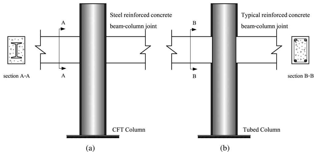
Figure 1. Two different composite columns: (a) Concrete filled steel tube column with steel reinforced concrete beam-column joint and (b) Tubed column with typical reinforced concrete beam-column joint
