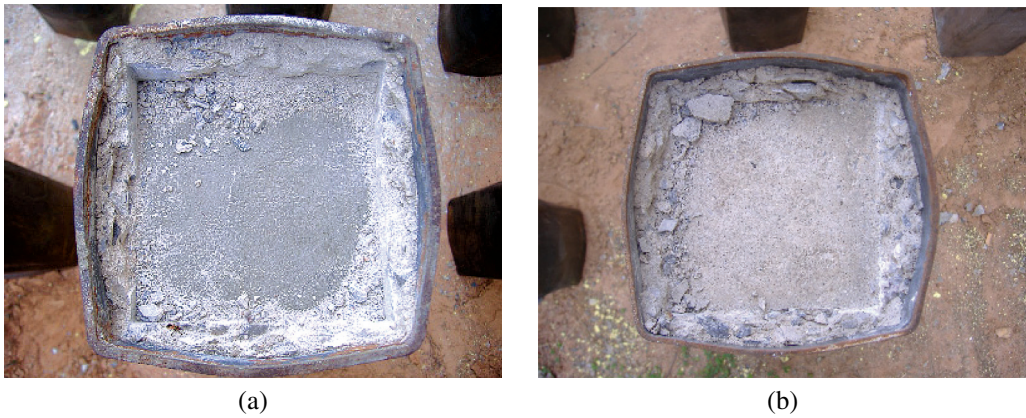
Figure 10. Failure mode of the RC core at the top of the tubed RC columns (a) t = 4.5 mm, (b) t = 3.2 mm
